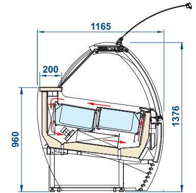
MITO POWER 12, 16, 18, 20, 24
